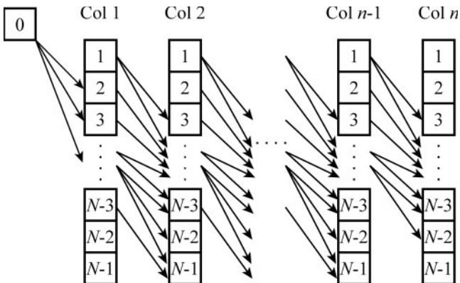
Fig. 2. SDR as a shortest-path problem. Every feasible n -crossover library can be represented as an n -path from node 0 to column n . The node visited in column k corresponds to the position of the k th crossover, shown here for a protein of length N . To constrain the length of each peptide fragment, nodes in adjacent columns are selectively connected. Arc lengths are assigned so that the total path length of each n -path equals the average energy of the corresponding library (see Results).
