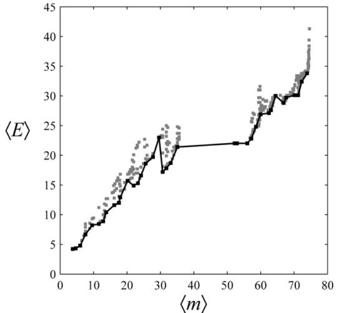
Fig. 3. The energy-diversity tradeoff for RASPP libraries. Equation 1 was solved with cytochrome P450 homologs CYP102A1/A2/A3 ( n = 7 crossovers, N = 197 non-conserved residues) for length constraints L_{\min} = 1 to N/(n+1) and L_{\max} = N/(n+1) to N - nL_{\min} . A plot of \langle E \rangle versus \langle m \rangle for the 391 distinct libraries in this set (gray squares) reveals that no RASPP libraries fall in the range 40 < \langle m \rangle < 50 . This is a consequence of using constraints on fragment length as a surrogate for \langle m \rangle . The 'RASPP curve' (black line) was generated by dividing the \langle m \rangle -axis into bins of 1.5 mutations and keeping the lowest energy library within each bin (black squares).
