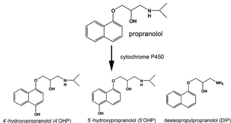
Figure 1. Major metabolites of propranolol formed by human cytochromes P450.
